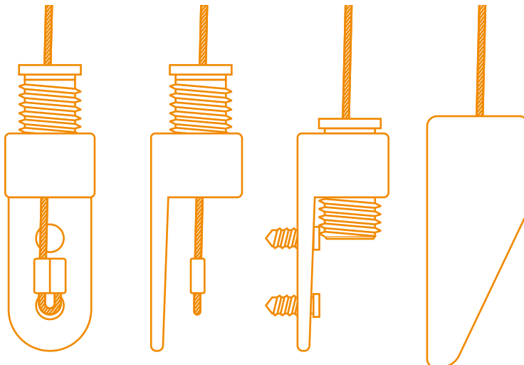
VISTA FRONTAL
